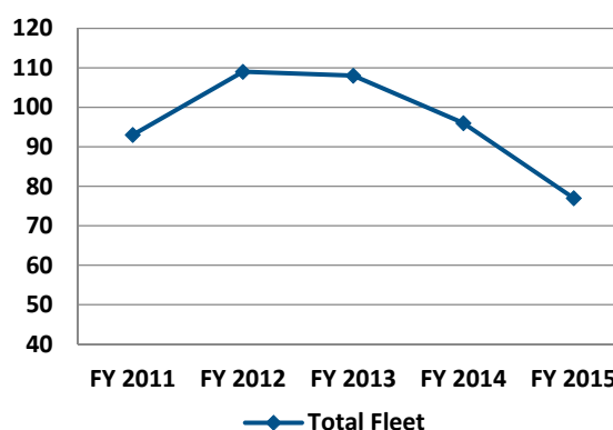
Figure 1-10: Total Fleet, 2011–2015
