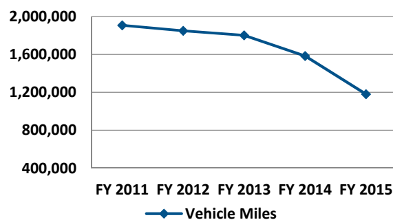
Figure 1-8: Vehicle Miles, 2011–2015
