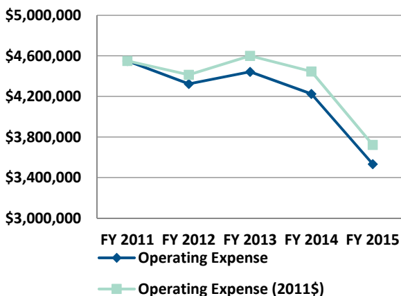
Figure 1-11: Operating Expense, 2011–2015
