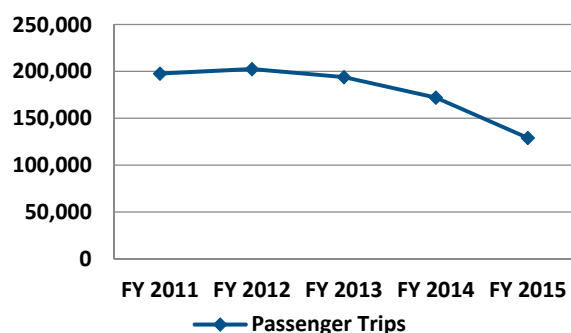
Figure 1-7: Passenger Trips, 2011–2015
