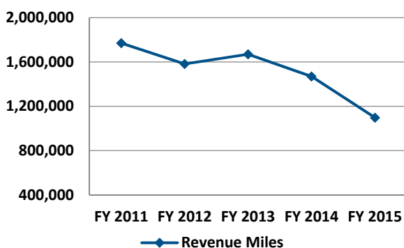
Figure 1-9: Revenue Miles, 2011–2015
